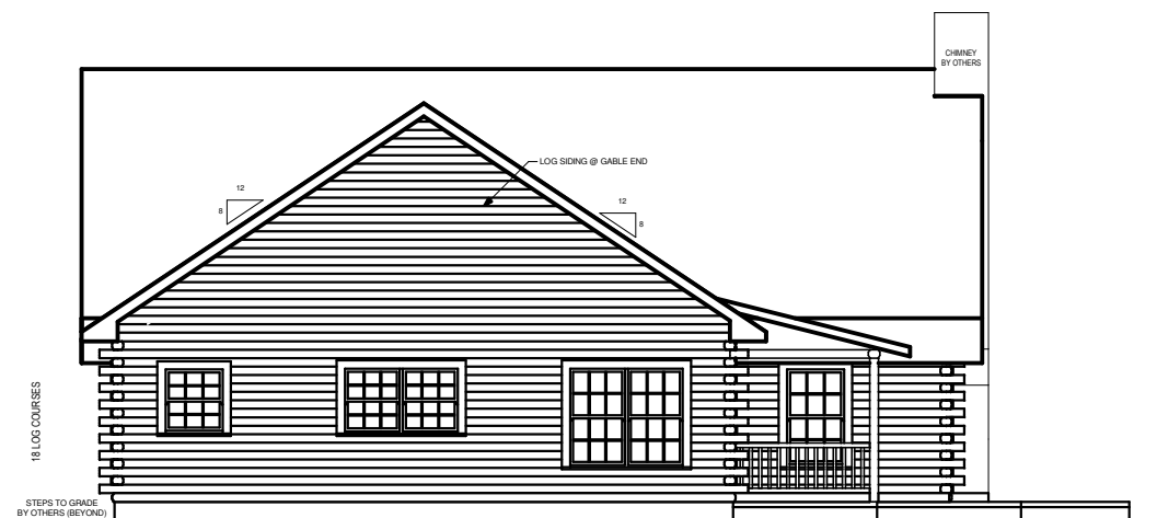
LEFT ELEVATION
