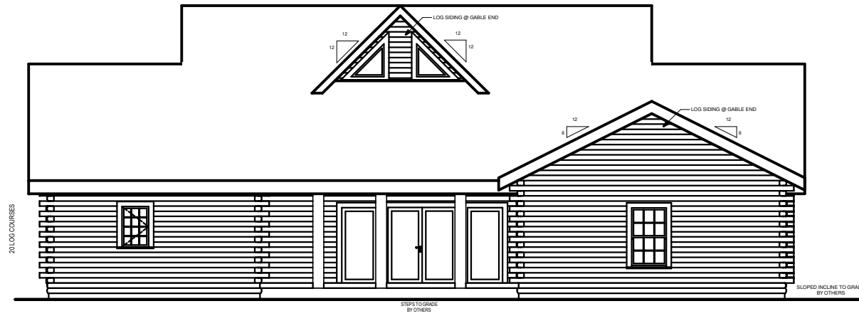
REAR ELEVATION
