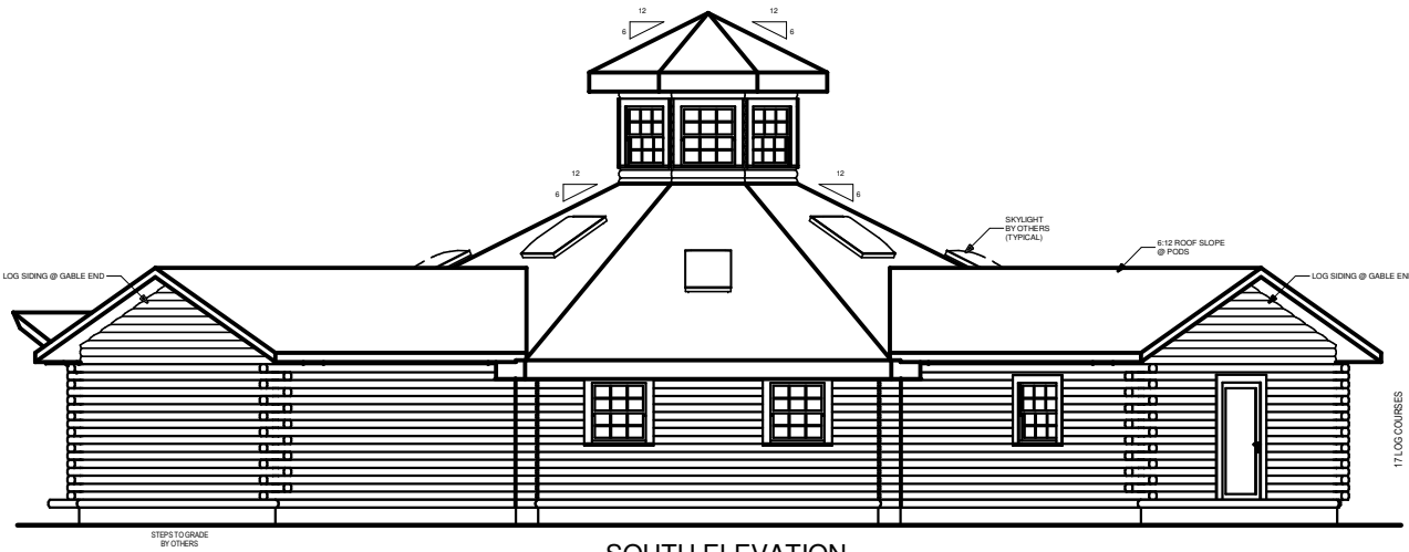
SOUTH ELEVATION
