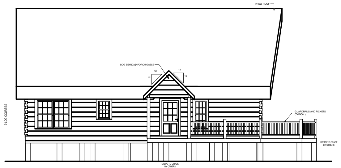
LEFT ELEVATION
