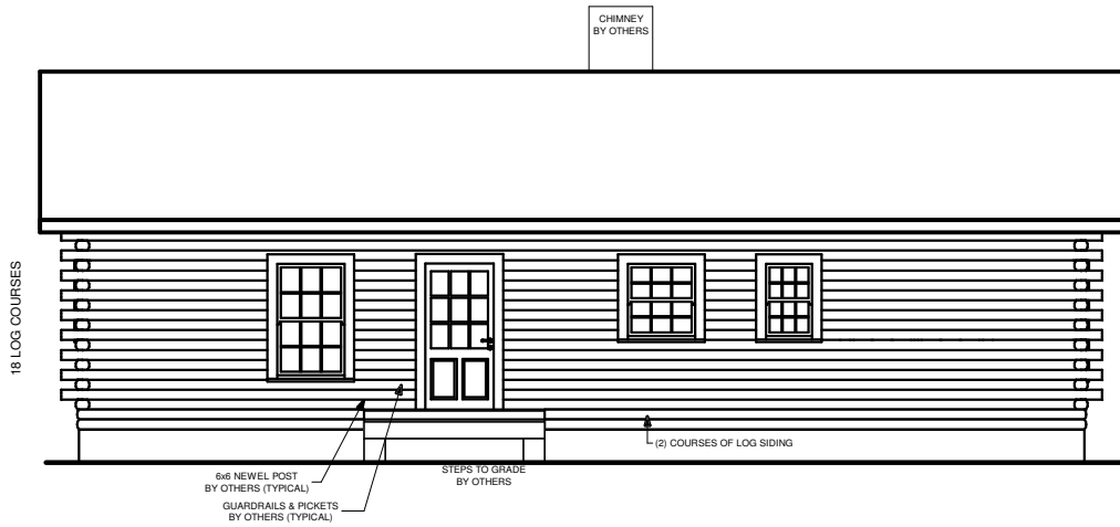
REAR ELEVATION
