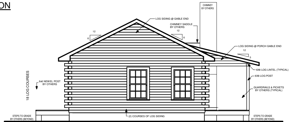
LEFT ELEVATION
