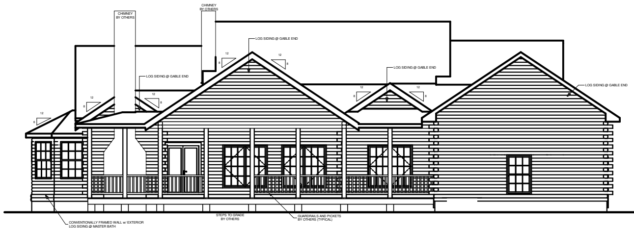
REAR ELEVATION
