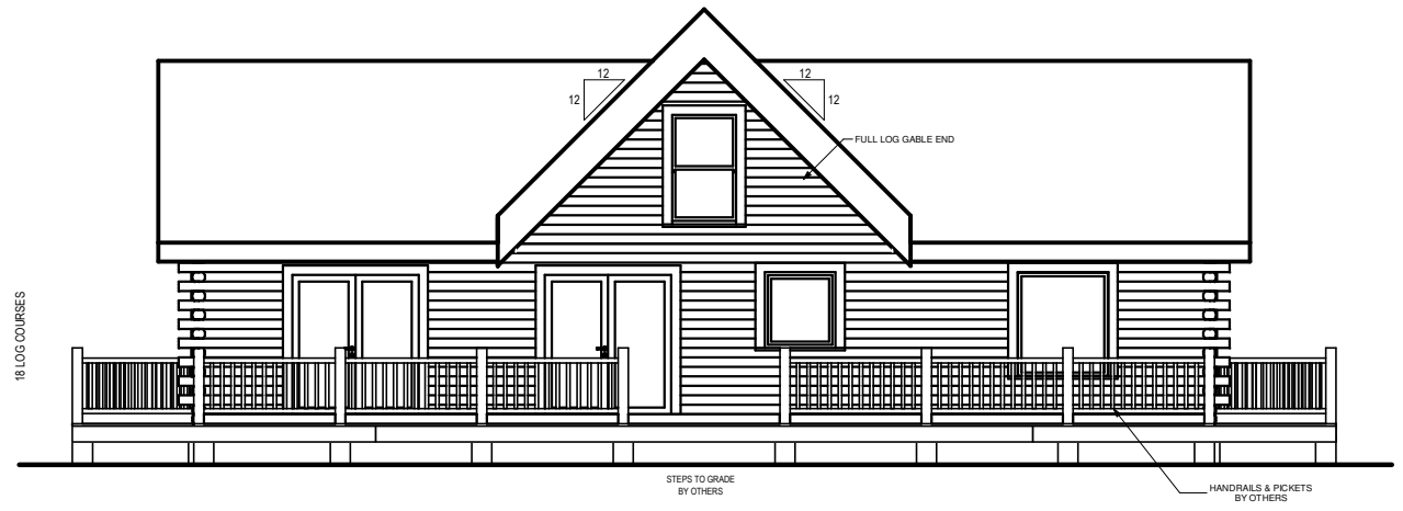
REAR ELEVATION
