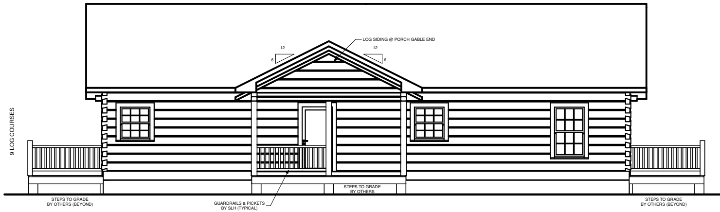
REAR ELEVATION
