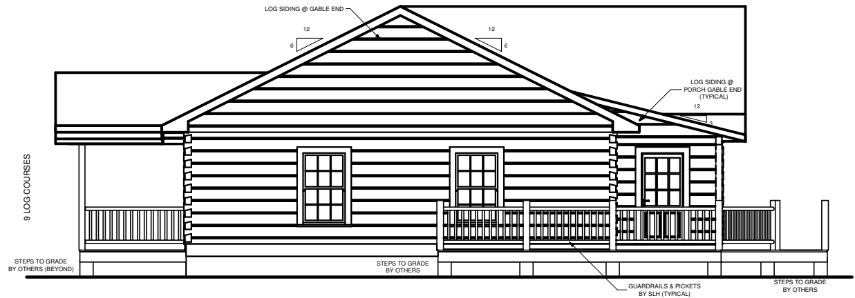
LEFT ELEVATION
