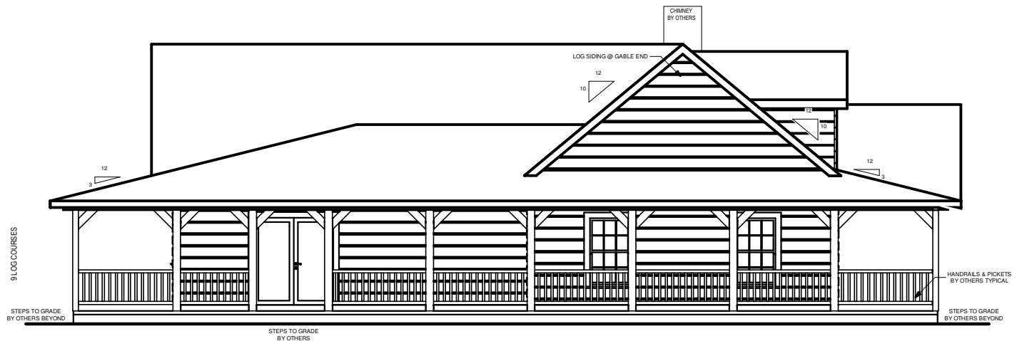
LEFT ELEVATION
