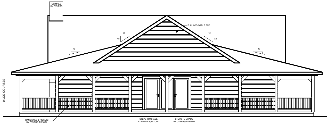
REAR ELEVATION
