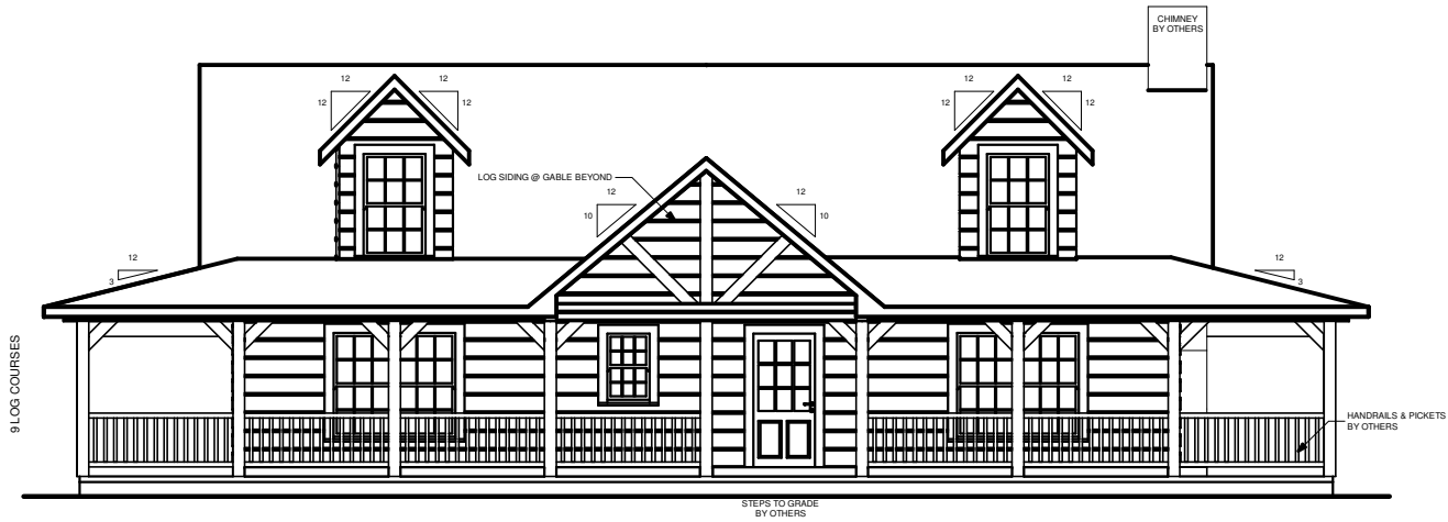
FRONT ELEVATION
