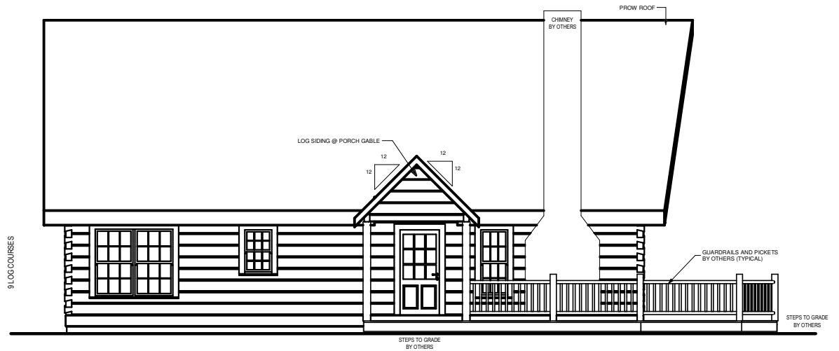
LEFT ELEVATION
