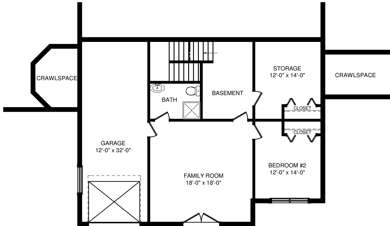
BASEMENT PLAN
