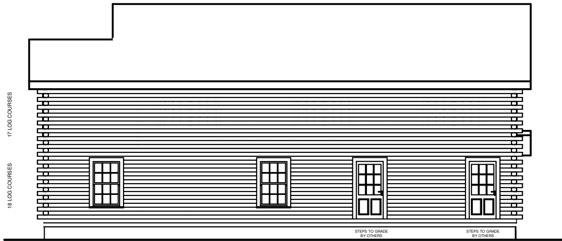
REAR ELEVATION
