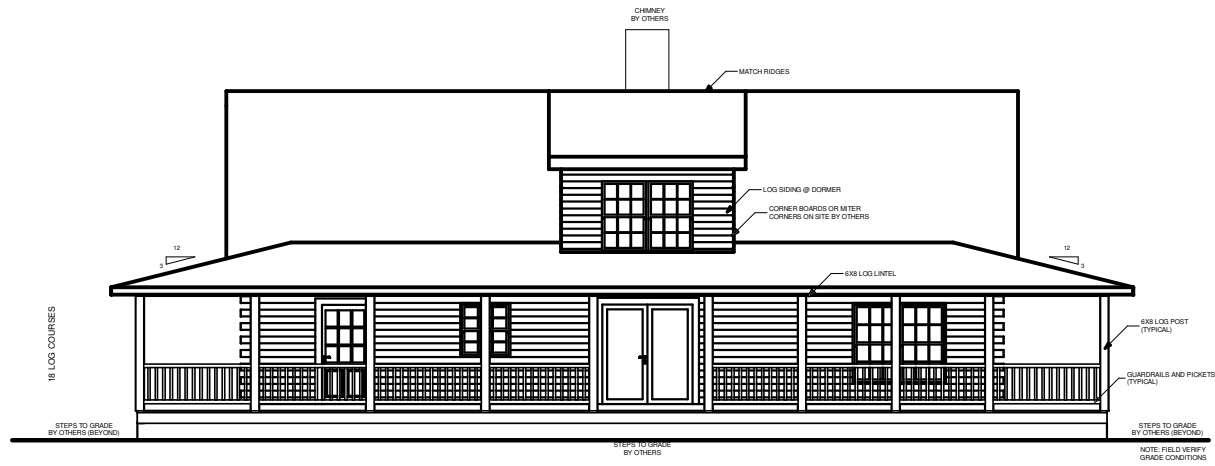
REAR ELEVATION 1/4" = 1'-0"
