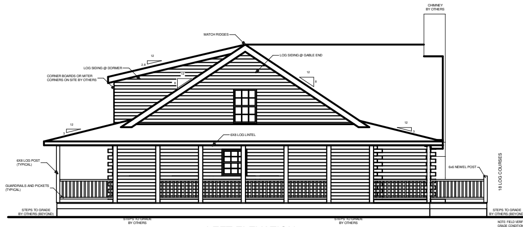
LEFT ELEVATION 1/4" = 1'-0"
