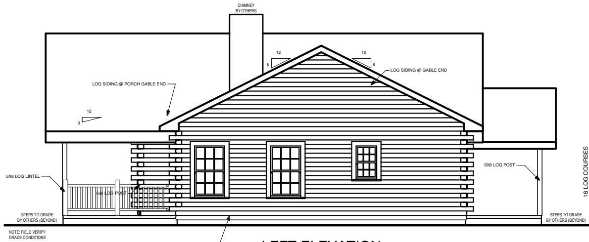
LEFT ELEVATION
