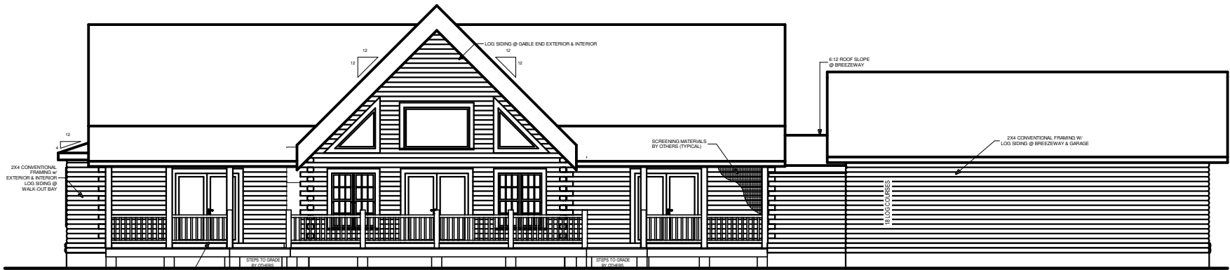
REAR ELEVATION
