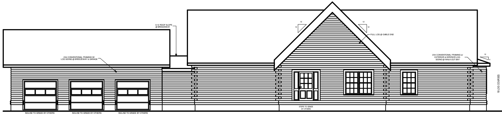
FRONT ELEVATION
