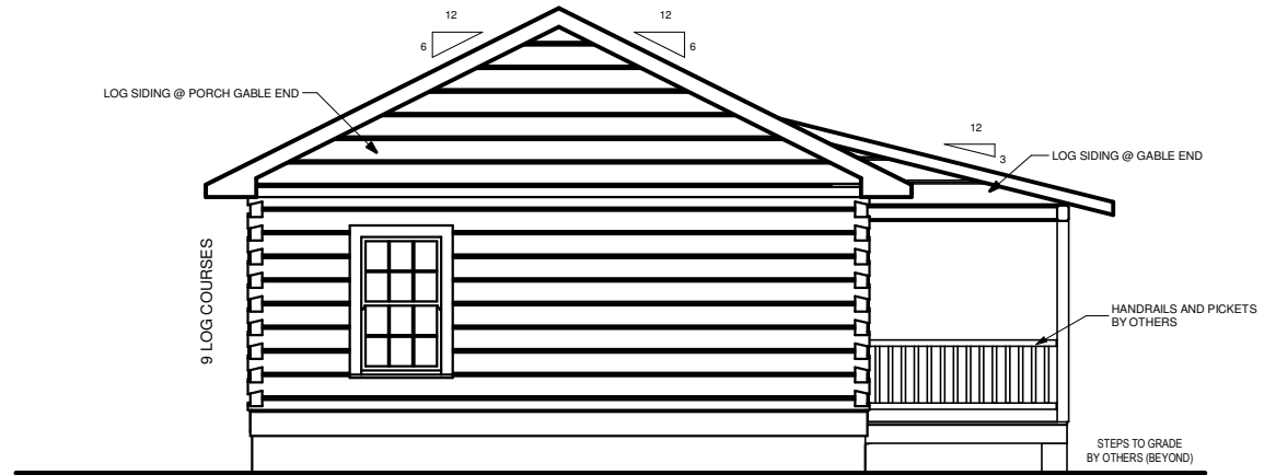
LEFT ELEVATION
