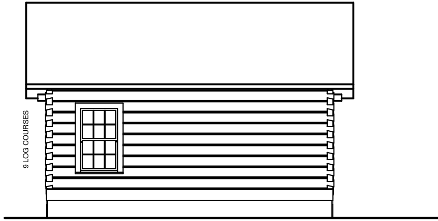
REAR ELEVATION
