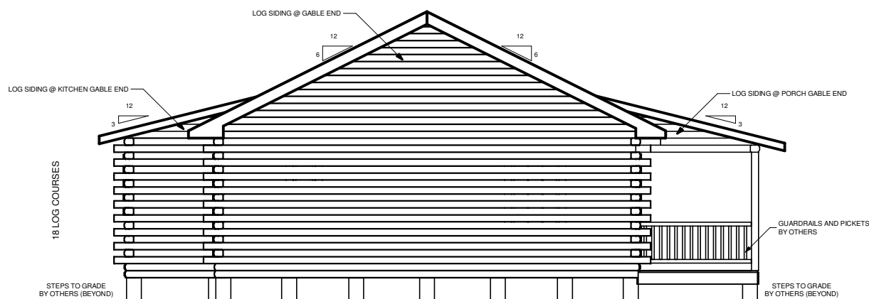
LEFT ELEVATION
