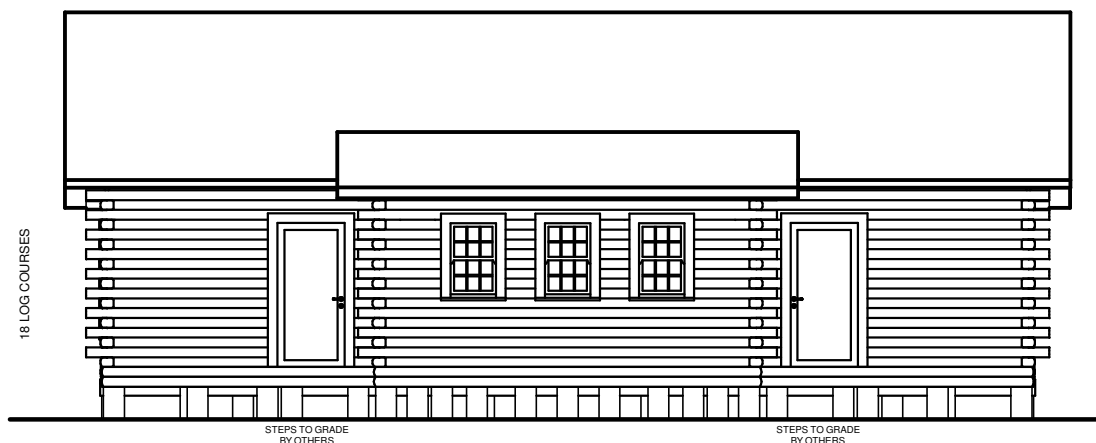
REAR ELEVATION
