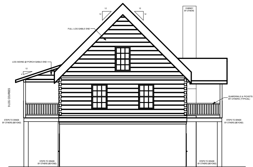
REAR ELEVATION
