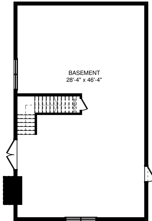
BASEMENT PLAN
