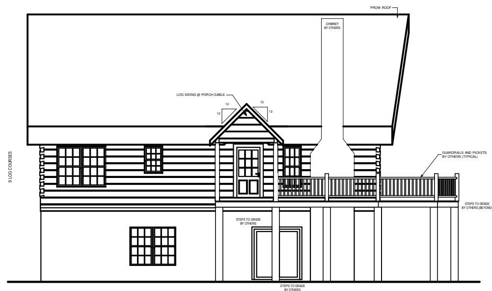
LEFT ELEVATION
