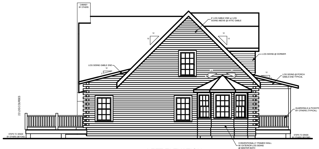
LEFT ELEVATION
