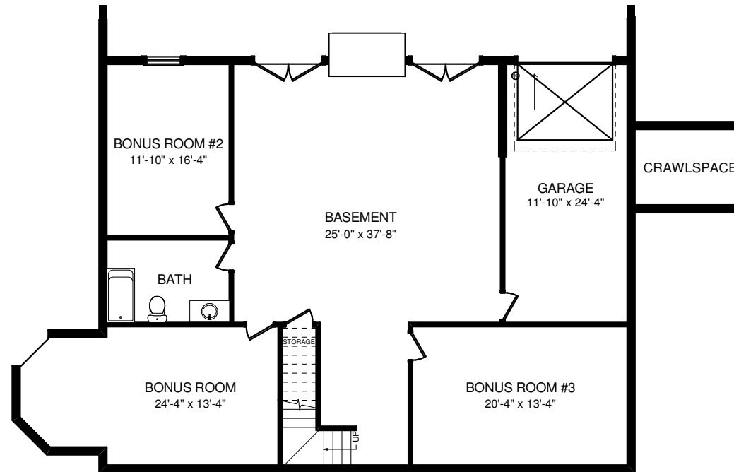
BASEMENT PLAN
