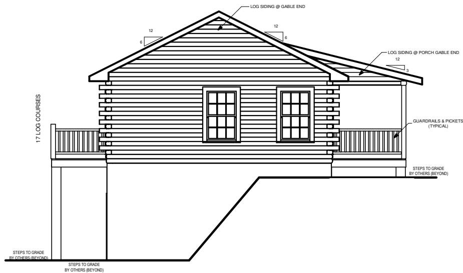
LEFT ELEVATION
